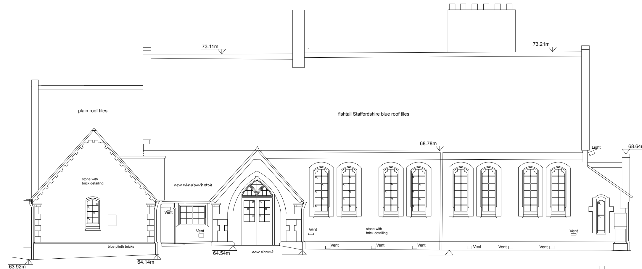
South Elevation
