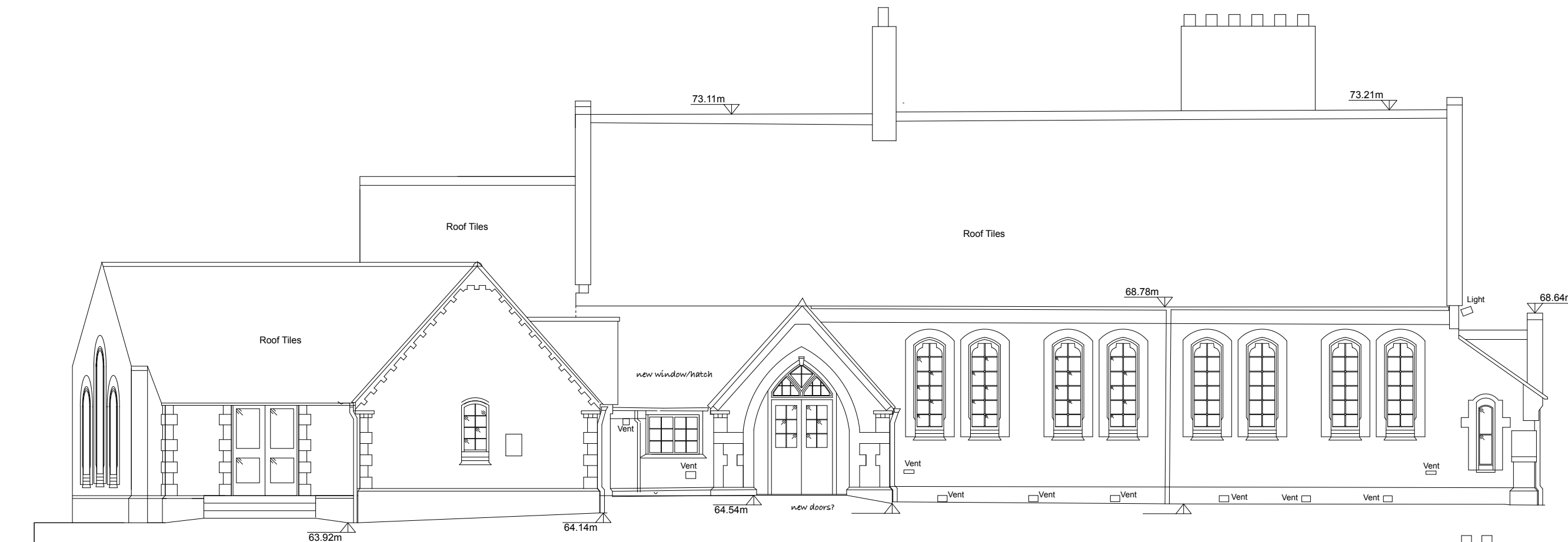
South Elevation
