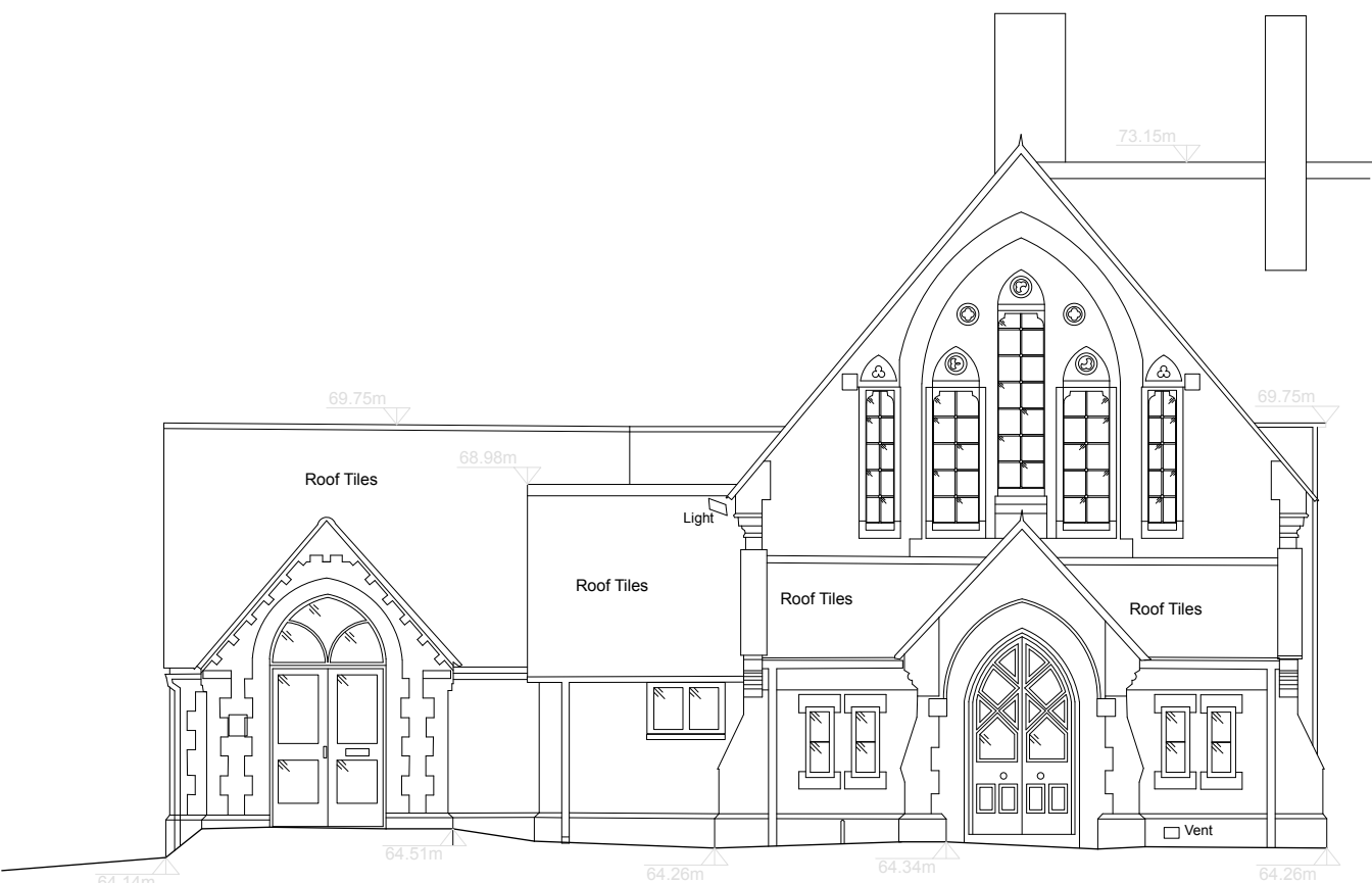
East Elevation
